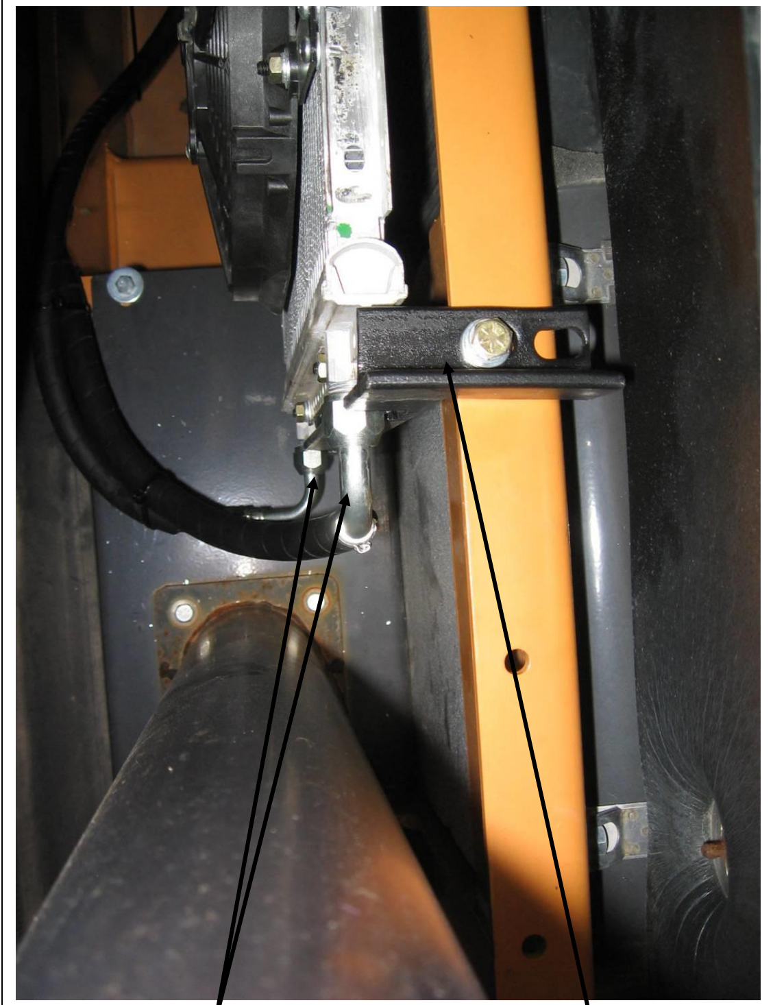
Condenser hoses connected using 90° fittings at top and bottom.
