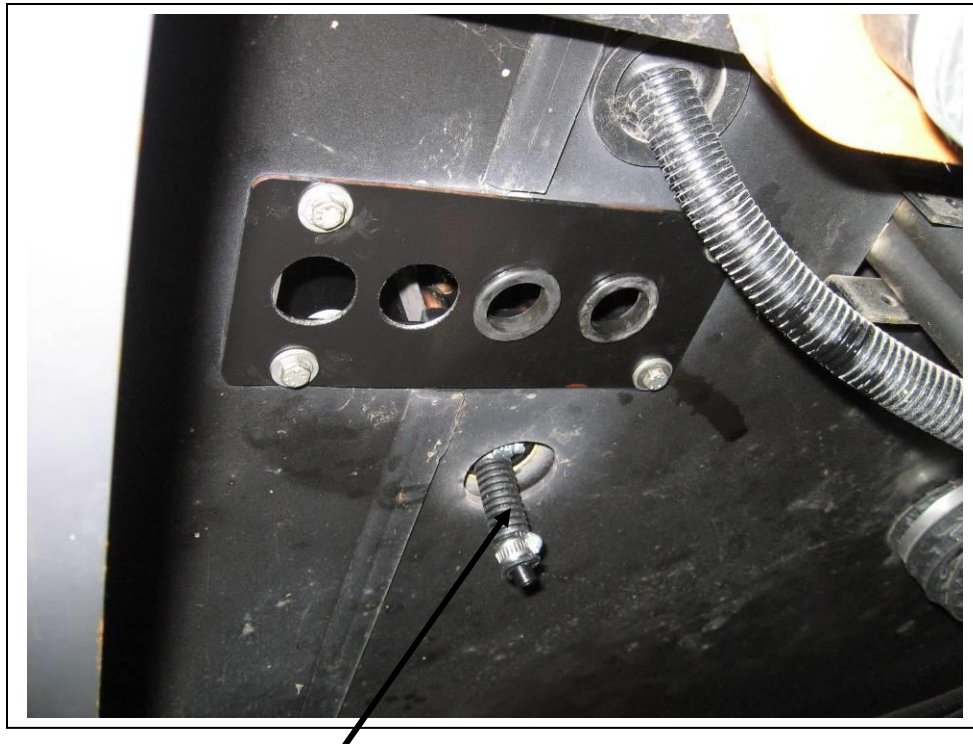
Short drain tubes and drain restrictors installed.
