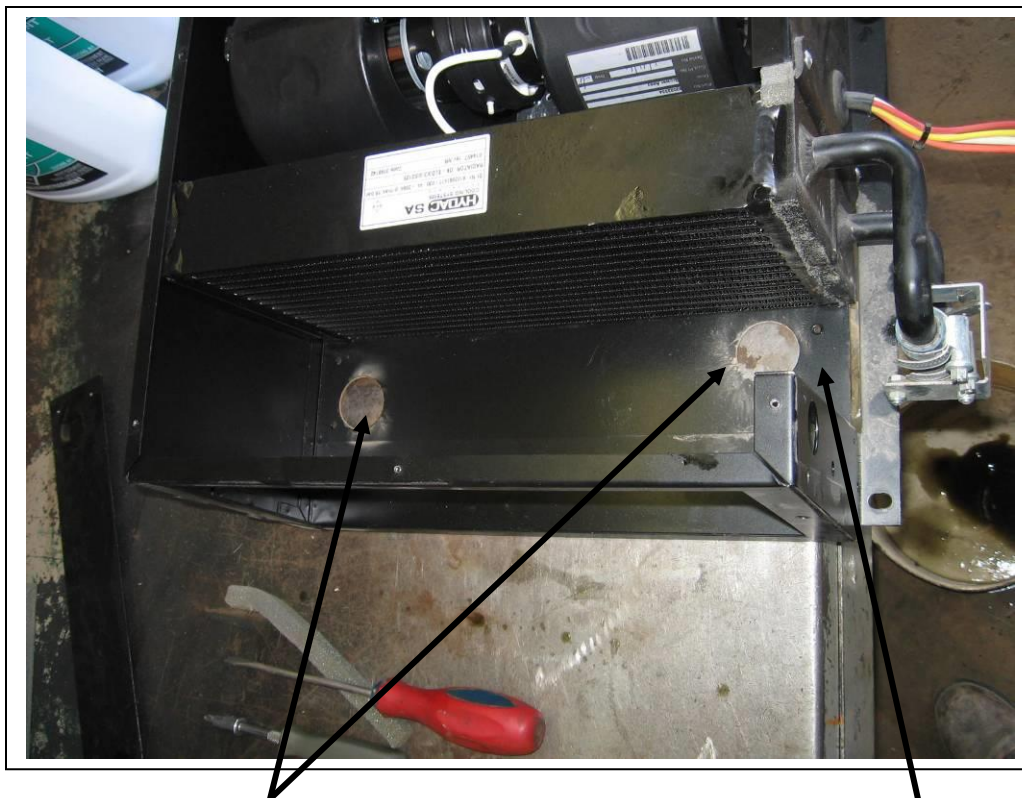
Remove drain plugs
