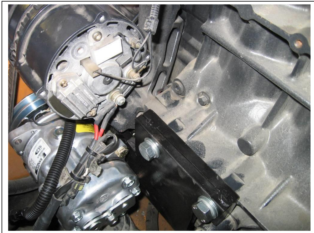
Install compressor and mount as shown.
