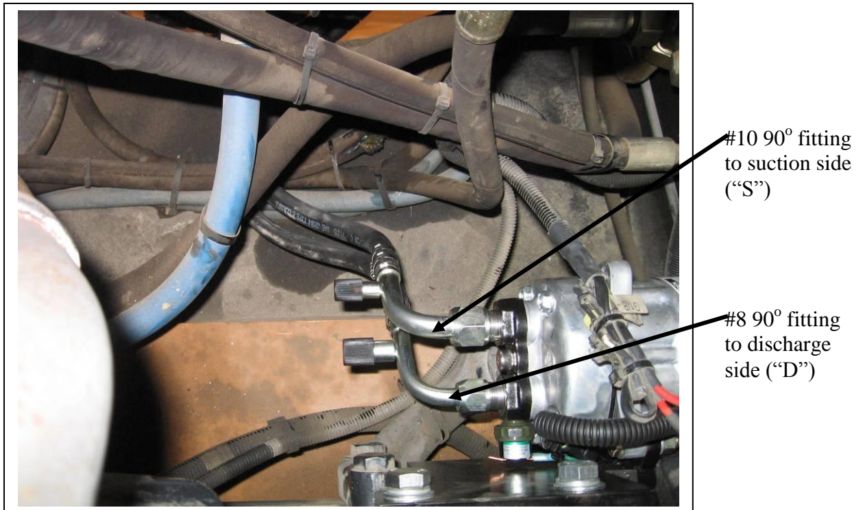
View from the top with hoses connected to the compressor pad.
